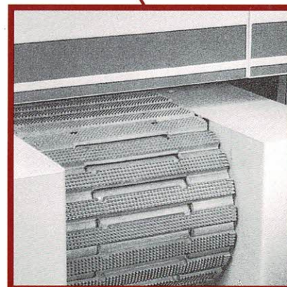
Transportkette - keine Einschlüsse durch geschlossene Transportkette - exakter Werkstücktransport Transport Chain - No material between links with closed transport chain - accurate and parallel board feed
